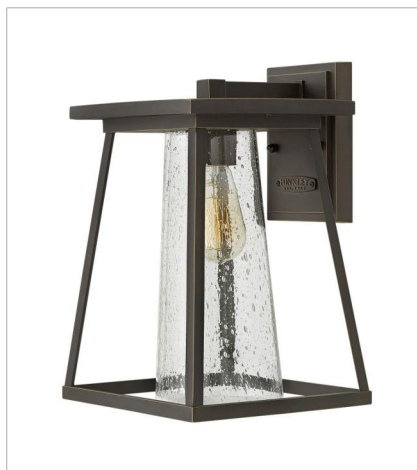
2794OZ-CL MEDIUM WALL MOUNT LANTERN 9" W, 14" H Socketed 1-10w Med. LED, 100w Equiv.
