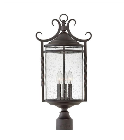
1141OL-CL LARGE POST TOP OR PIER MOUNT LANTERN 12" W, 23.8" H Socketed 3-5w Cand. LED, 60w Equiv.
