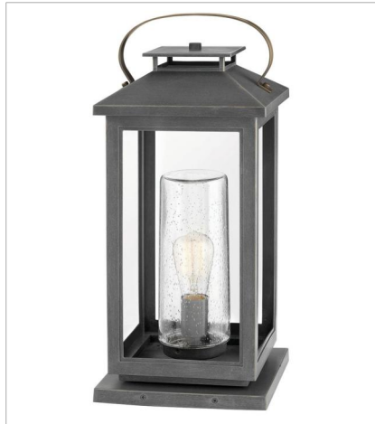
1167AH-LV LARGE PIER MOUNT LANTERN 12V 9.5" W, 21.5" H Socketed 1-3.50w Med. LED *Included
