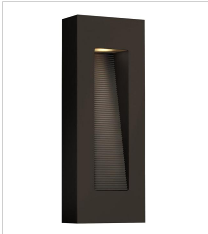
1668BZ MEDIUM WALL MOUNT LANTERN 6" W, 16.3" H Socketed 2-7w GU10 LED, 20w Equiv.
