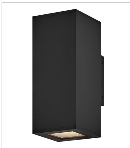
28914BK-LL SMALL WALL MOUNT LANTERN UP... 5" W, 12" H Socketed 2-7w GU10 LED *Included
